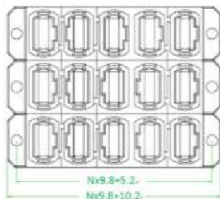
MPO STACKABLE ADAPTER, STRAIGHT TYPE, M x N
