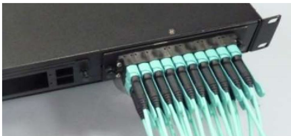
MPO STACKABLE ADAPTER, STRAIGHT TYPE, M x N
