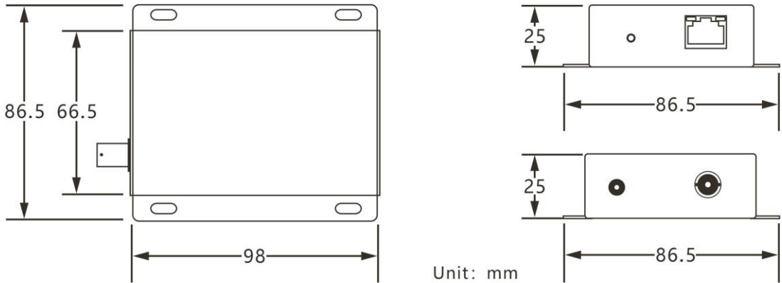
Receiver Unit
