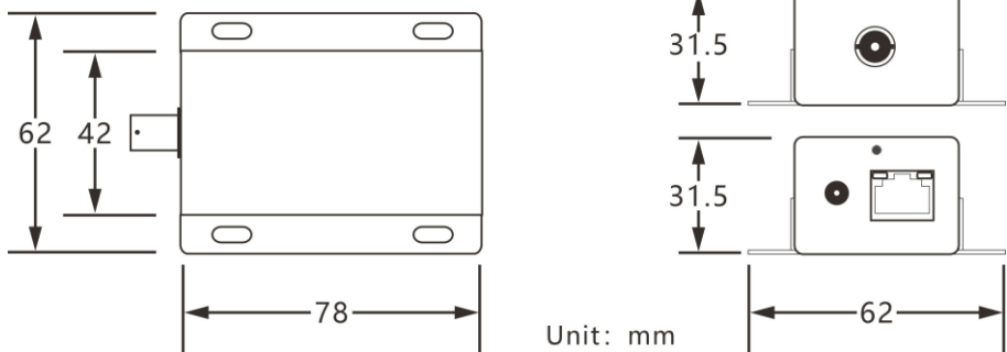
Transmitter Unit
