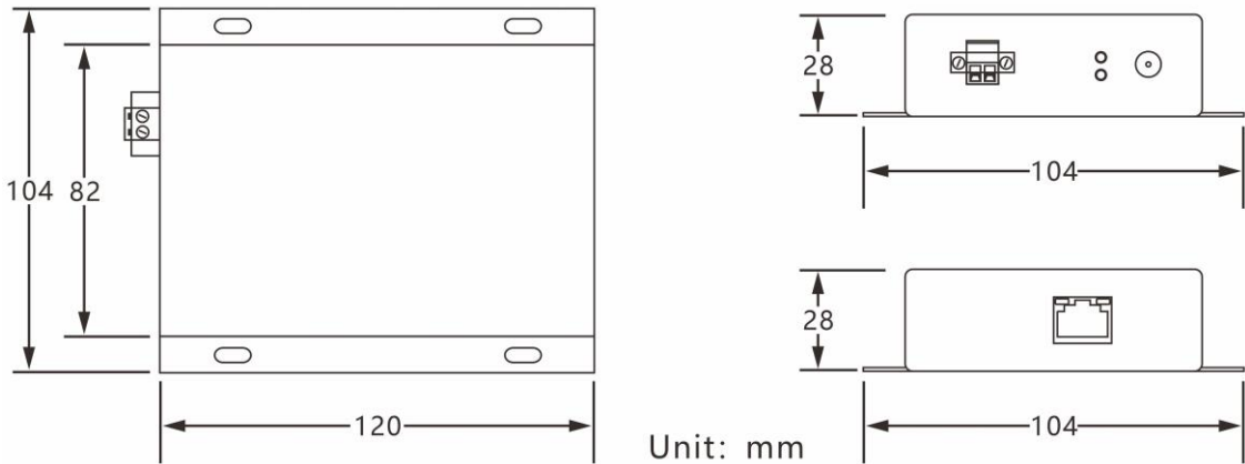
Receiver Unit
