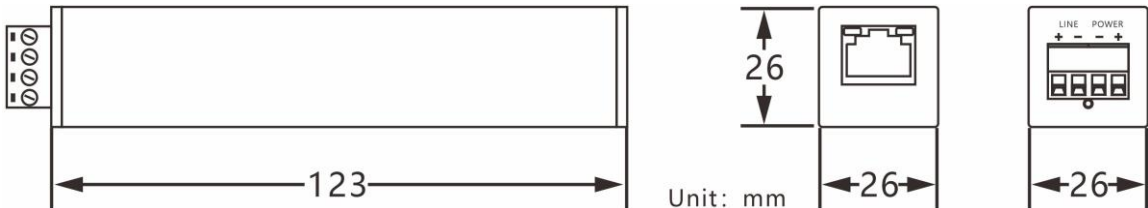
Transmitter Unit
