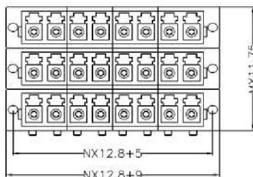
LC STACKABLE ADAPTER, STRAIGHT TYPE, M x N
